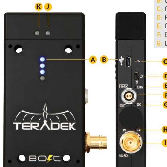
Bolt 3G-SDI Transmitter
